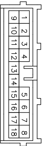
Front C (instrument harness and front compartment harness connecting pieces) (At the Right A Column)
