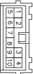
Ceiling Lamp (instrument harness and ceiling lamp harness connecting pieces)
